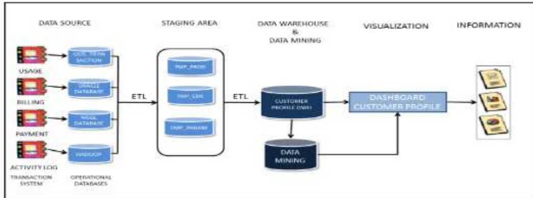
Figure 2 Data Architecture for Customer Profile
